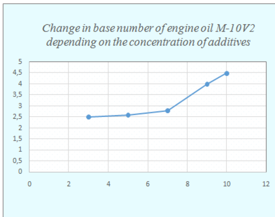
Fig 1. Physicochemical indicators of engine oil for various concentrations of additives
